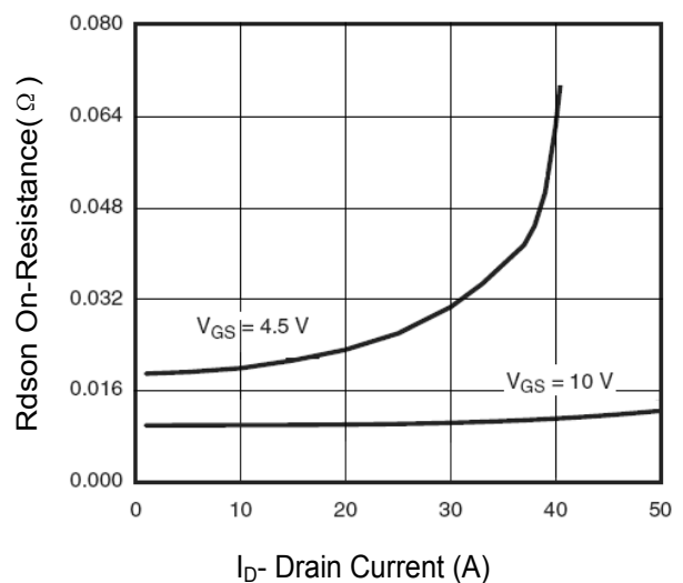
Figure 6 Drain-Source On-Resistance
